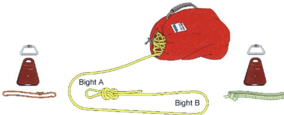
Figure 11-15: How to Construct a 3:1 Pig Rig
